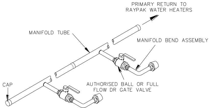
Heating Manifold Assembly
