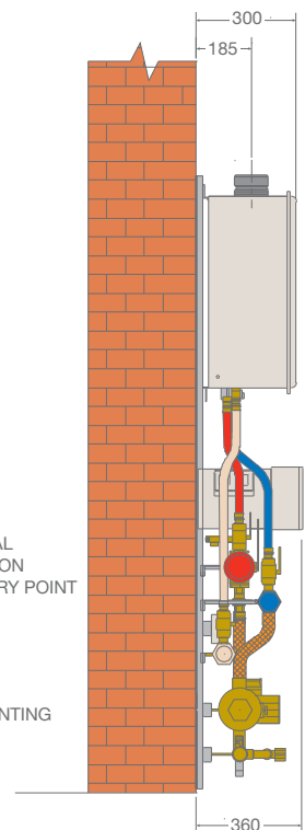
SIDE VIEW WALL MOUNTING
