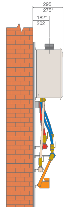
SIDE VIEW WALL MOUNTING
