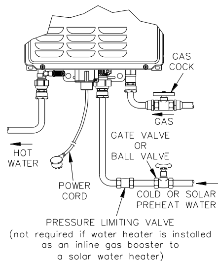
Gas Water Heater Cold (or Solar Heated) and Hot Water and Gas Connection Details
