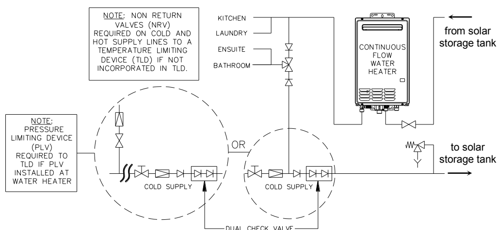
In-series Gas Booster as part of a Direct Solar Water Heater Installation Two Temperature Zones Using a Temperature Limiting Device
